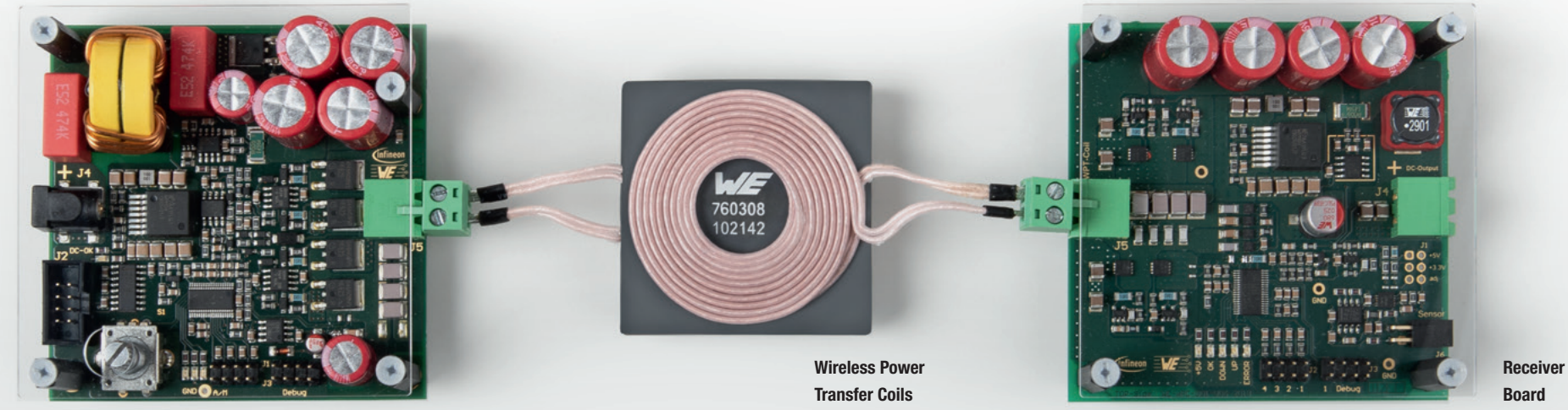
Transmitter Board
