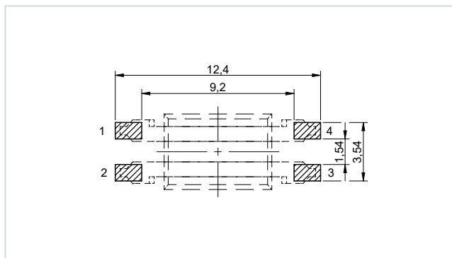
Recommended Land Pattern SLM: [mm]
