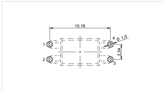
Recommended Hole Pattern M: [mm]
