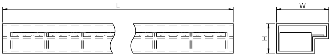
Figure 21: Packaging dimensions.
