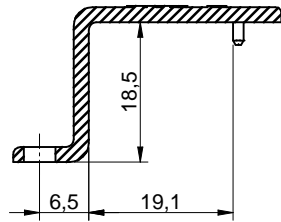
sectional drawing A-A
