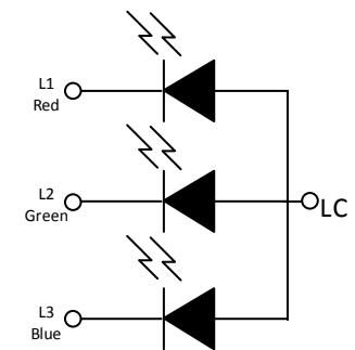
LED Schematic
