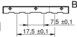
sectional drawing A-A
