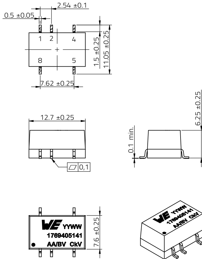
Figure 19: Physical dimensions.
