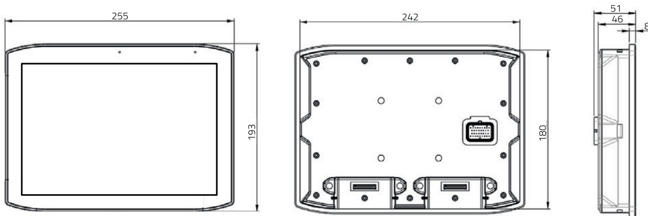
Dimensions – WEcabin Display i10 without buttons
