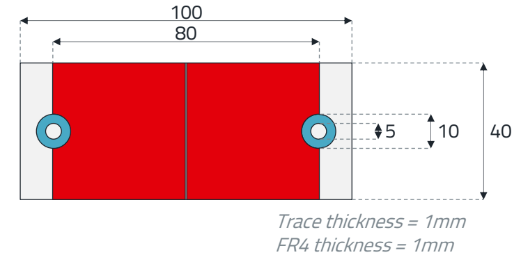
PCB Class D
