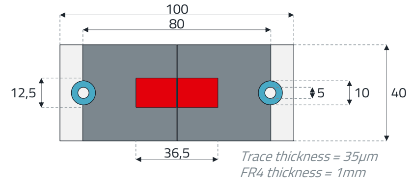
PCB Class B
