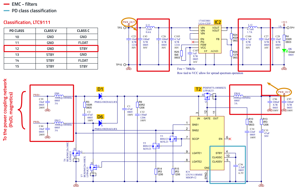
Figure 24: PoE-PD power supply with controller LTC9111.
