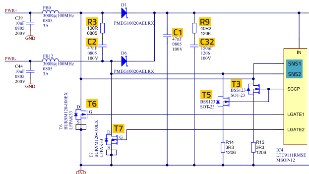
Figure 25: Section on left-hand side of the circuit shown in Figure 24.
