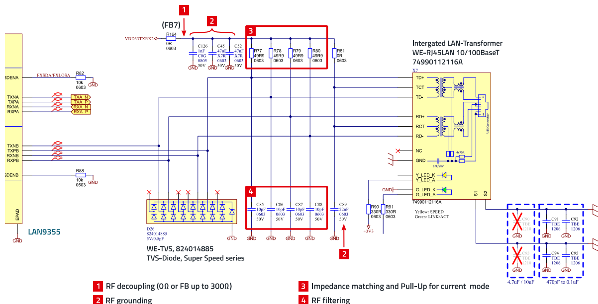
Figure 32: Ethernet port of the PD, with LAN switch LAN9355.
