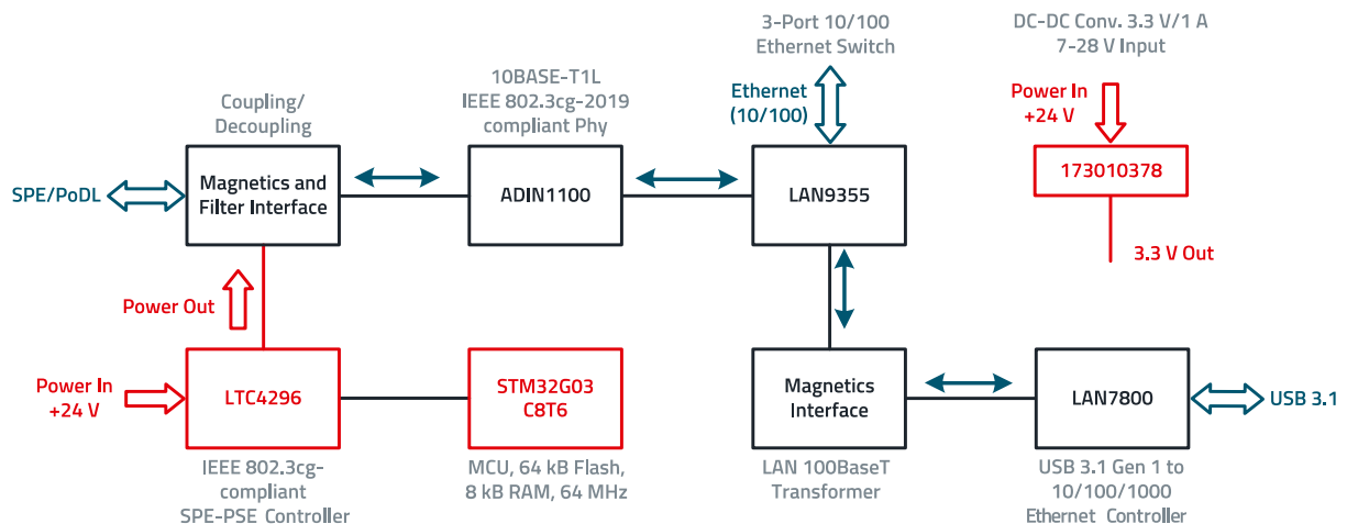
Figure 7: Block diagram of the PSE board.
