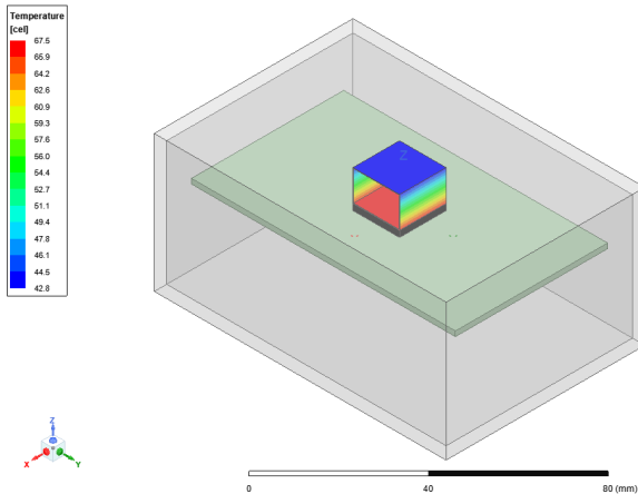
Abbildung 3: WE-TGFG-Simulation.
