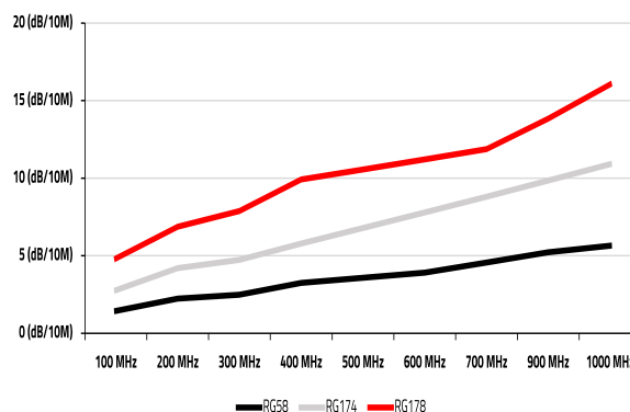
Figure 9: Cable attenuation overview
