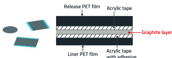
Figure 1: WE-TGS cross-section.
