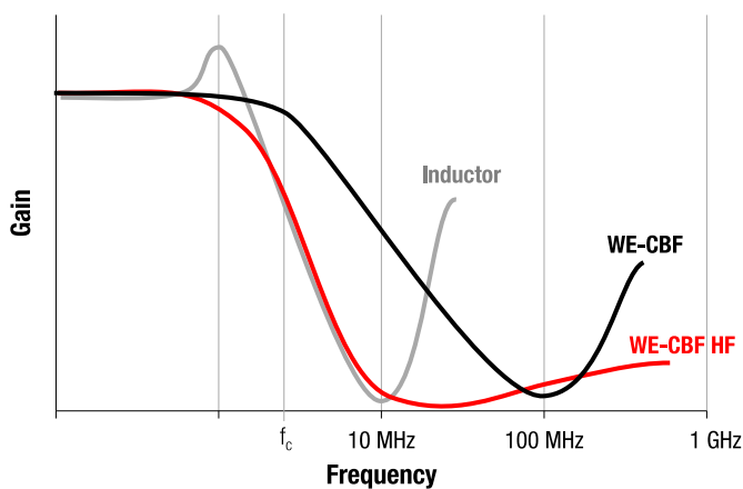
Figure 18: Gain response of a low pass filter for an inductor and ferrite beads.
