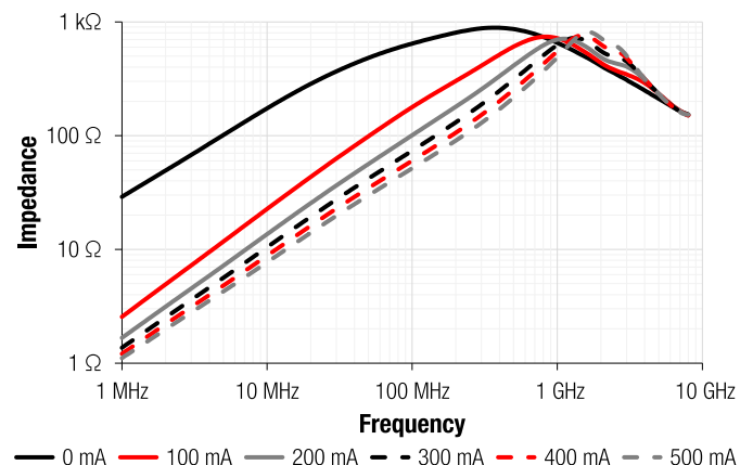
Figure 10: Comparison of the WE-CBF HF (742861160) under differing DC Bias conditions.
