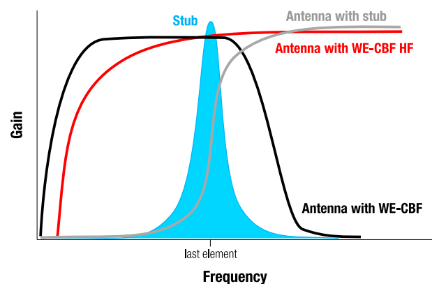
Figure 21: Gain over frequency of antenna with terminating stub
