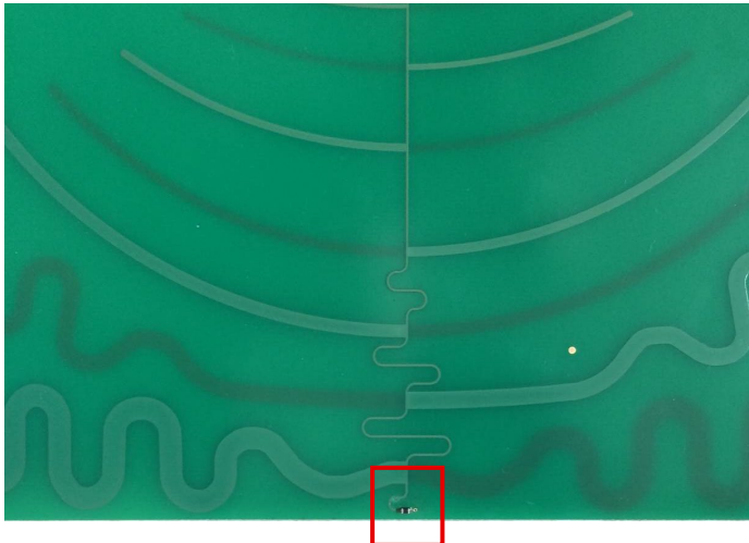
Figure 22: PCB of an LPDA with WE-CBF HF (742862160).
