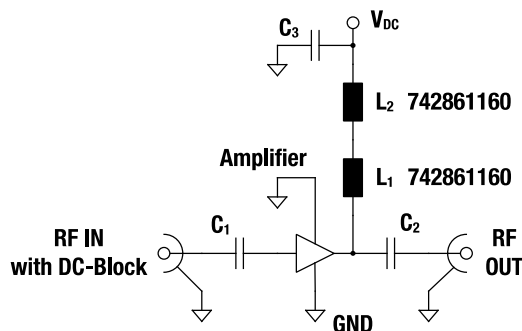
Figure 16: Gain amplifier circuit design.
