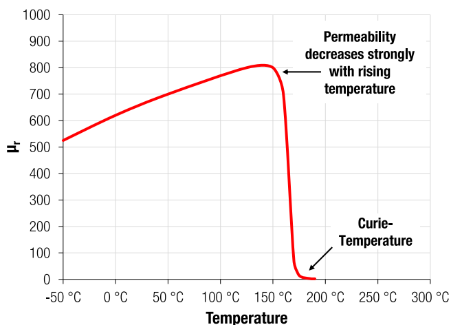
Figure 8: Curie temperature.
