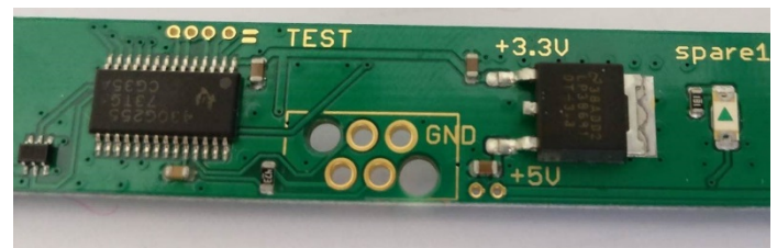
Figure 3: Layout and required space on the PCB
