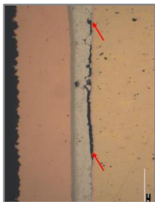
Cold solder joint
