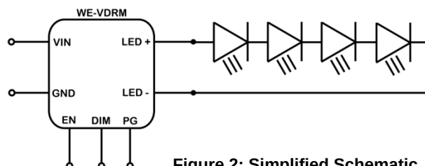
Figure 2: Simplified Schematic
