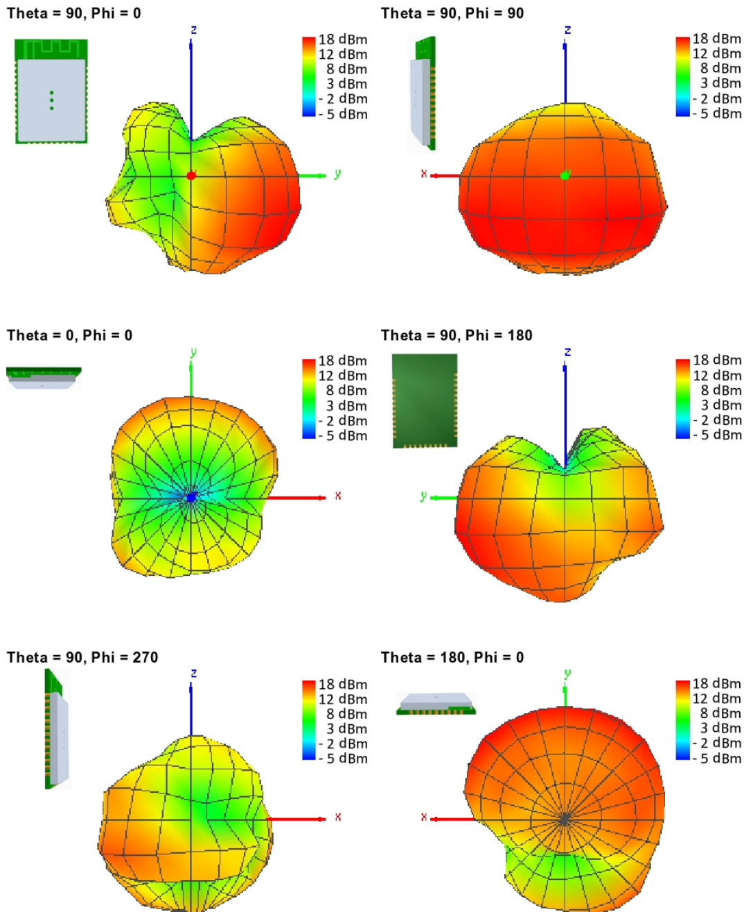
Figure 29: Antenna characteristic of the module with its integrated antenna measured on the official evaluation board
