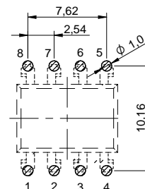
Recommended Hole Pattern M: [mm]
