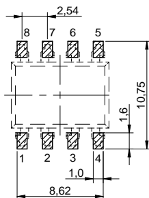
Recommended Land Pattern S: [mm]
