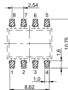
Recommended Land Pattern SL: [mm]
