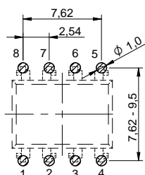
Recommended Hole Pattern Standard: [mm]
