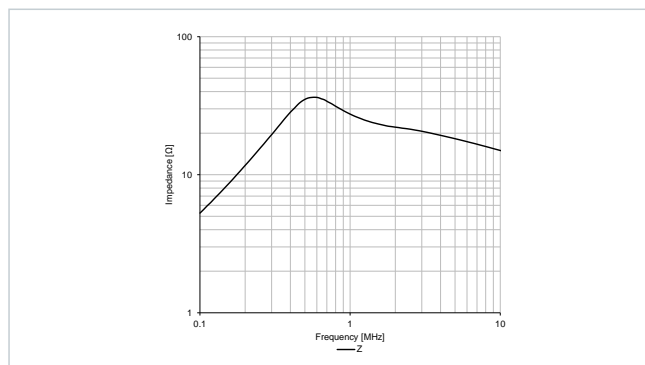
Typical Impedance Characteristics: 782115222150
