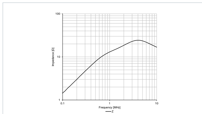
Typical Impedance Characteristics: 782115070080
