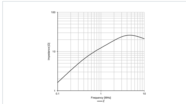
Typical Impedance Characteristics: 782115020030
