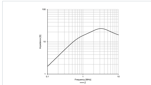
Typical Impedance Characteristics: 782115069064
