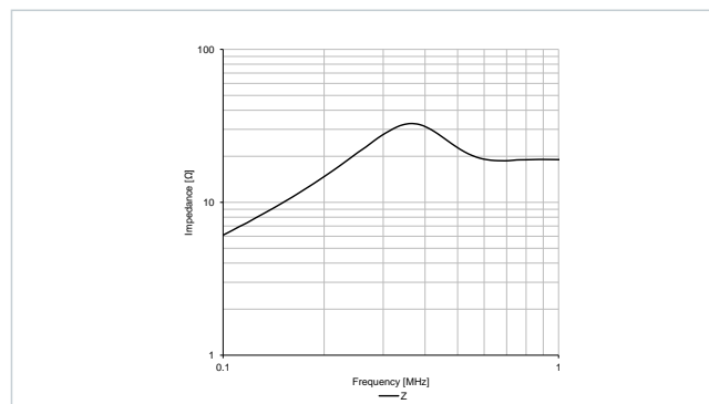
Typical Impedance Characteristics: 782115380150
