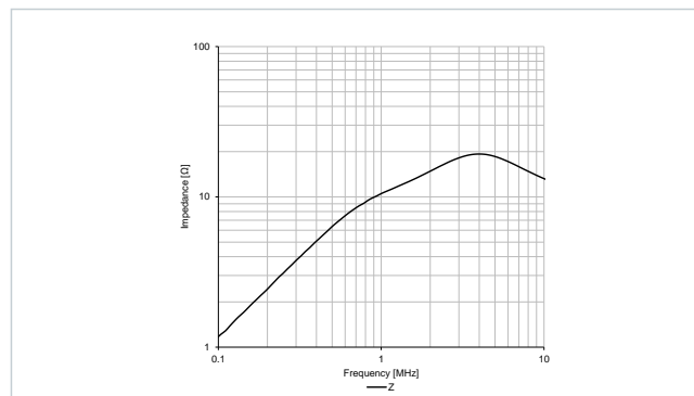
Typical Impedance Characteristics: 782115110070
