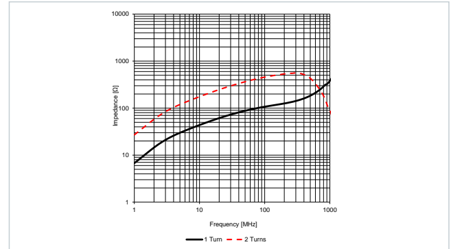
Typical Impedance Characteristics: 782114076130
