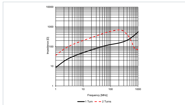
Typical Impedance Characteristics: 782114155200
