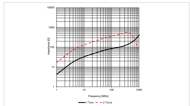
Typical Impedance Characteristics: 782114095100
