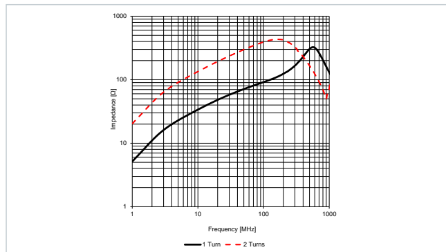
Typical Impedance Characteristics: 782114155130
