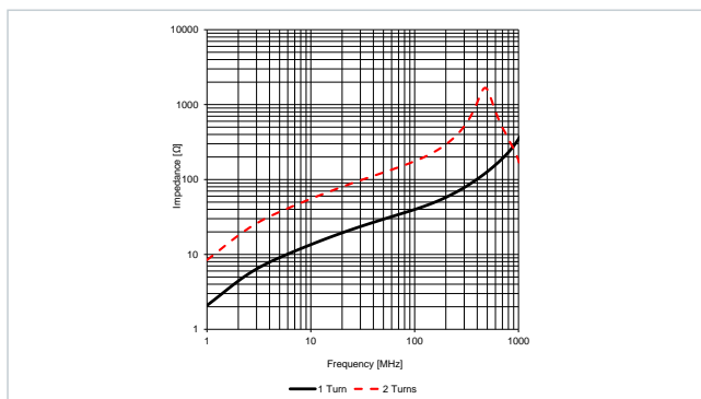
Typical Impedance Characteristics: 782114096080
