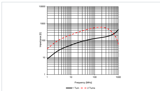
Typical Impedance Characteristics: 782114076160
