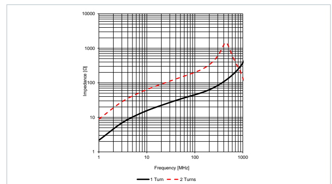
Typical Impedance Characteristics: 782114133064
