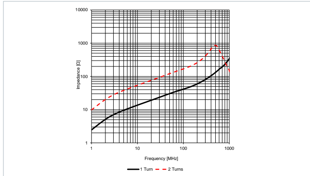
Typical Impedance Characteristics: 782114075063
