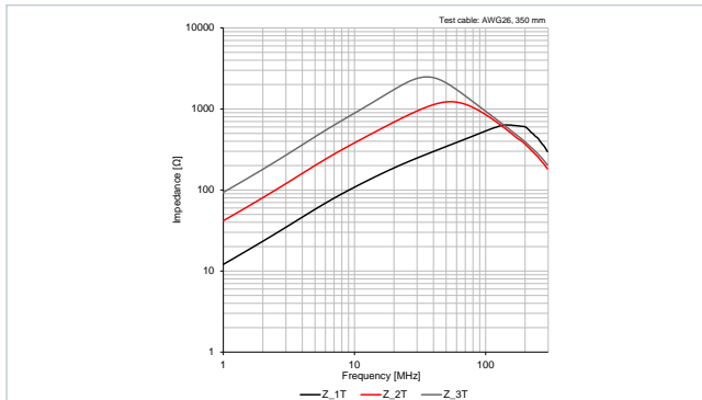
Typical Impedance Characteristics: 78271111(S)
