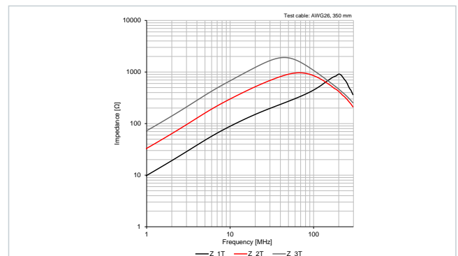
Typical Impedance Characteristics: 78271132(S)
