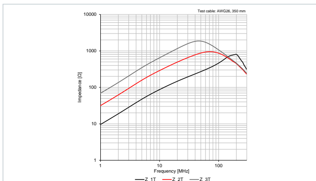
Typical Impedance Characteristics: 78271131(S)
