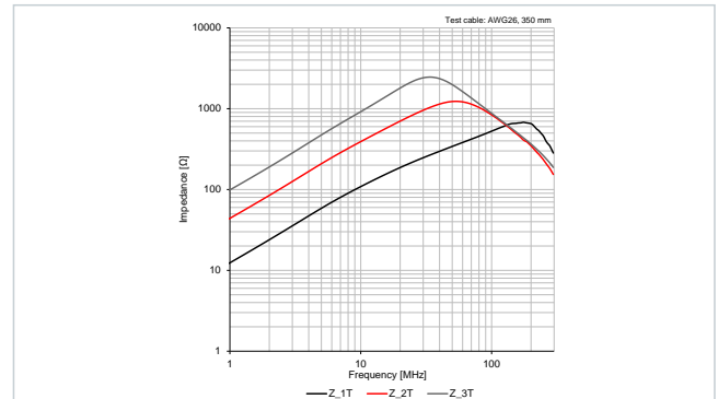
Typical Impedance Characteristics: 78271112(S)
