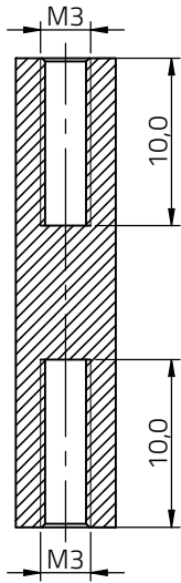
sectional drawing A-A
