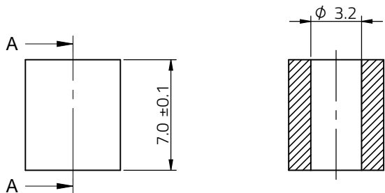
sectional drawing A-A
