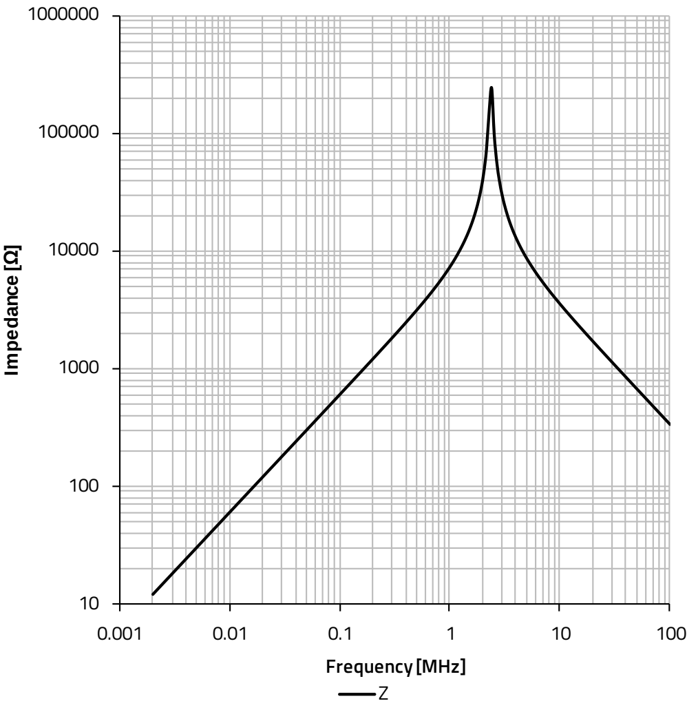
Typical Impedance vs. Frequency:
