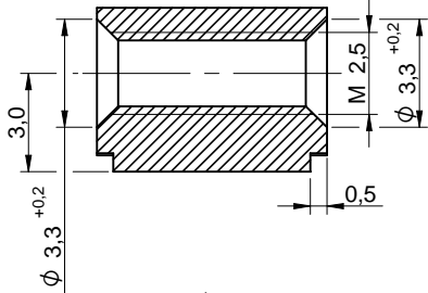
sectional drawing A-A
