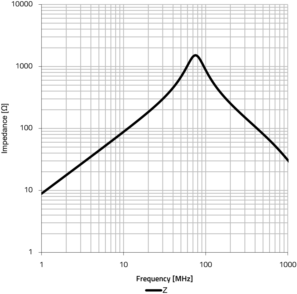
Typical Impedance vs. Frequency Characteristics:
