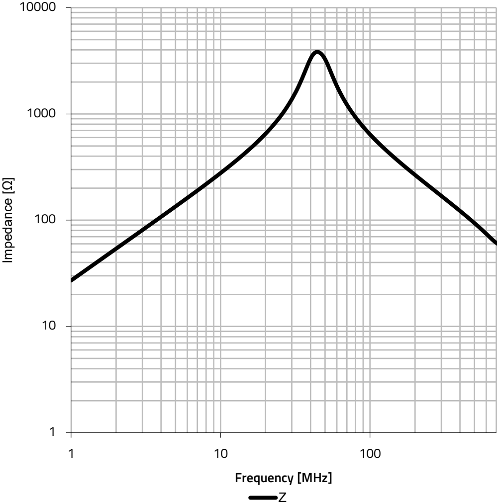
Typical Impedance vs. Frequency Characteristics:
