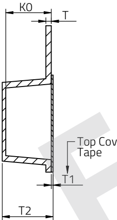
sectional drawing A-A
