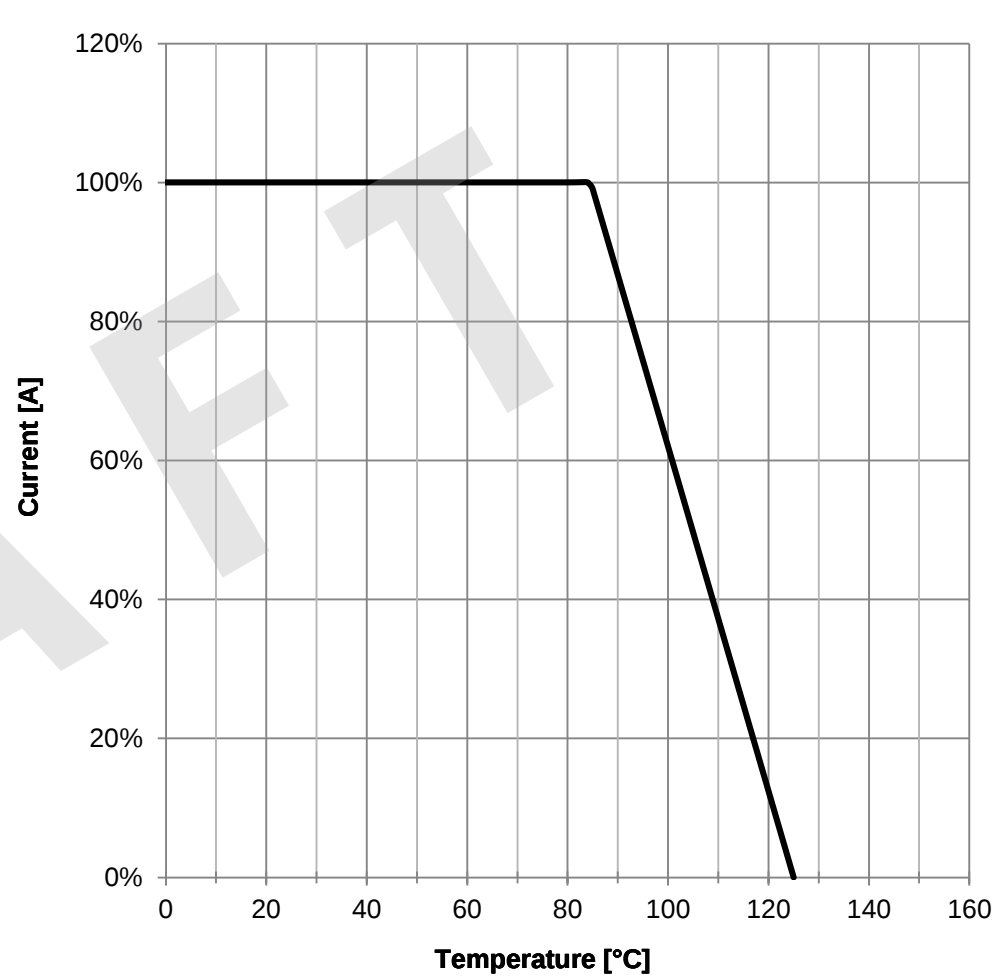
Derating Curve:
