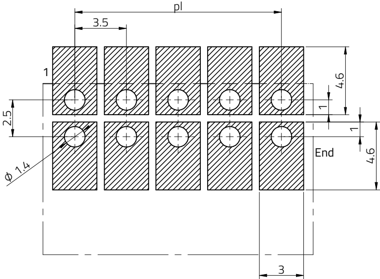
Stencil thickness : 120µm
