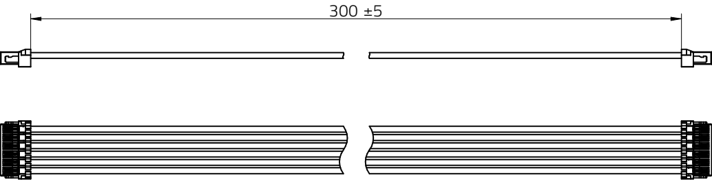
Connector 6890xx114322
