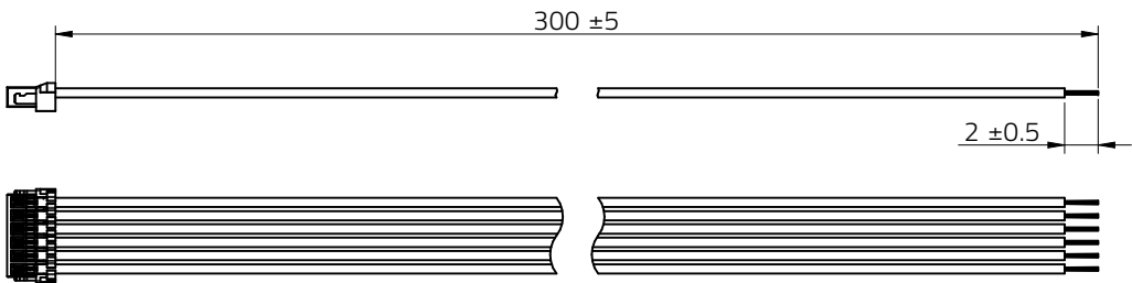
Connector 6890xx114322
