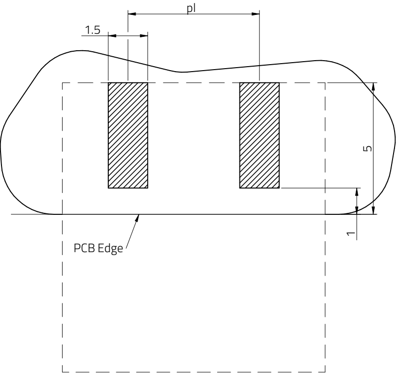
Recommended layout only for coding OA
