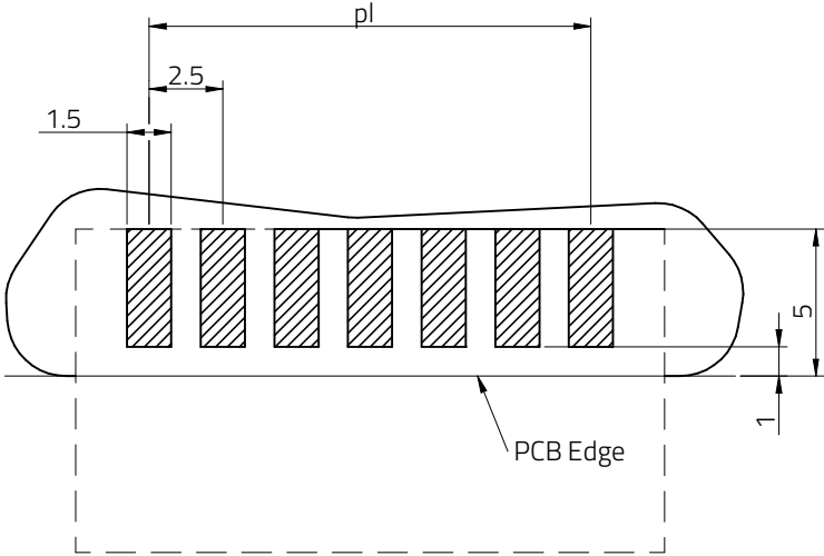
Recommended layout only for coding OA
