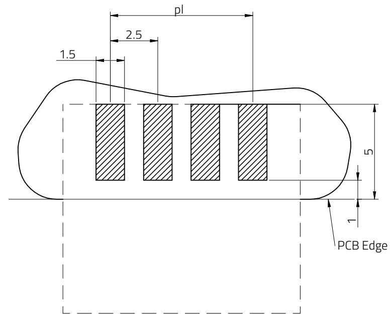
Recommended layout only for coding OA
