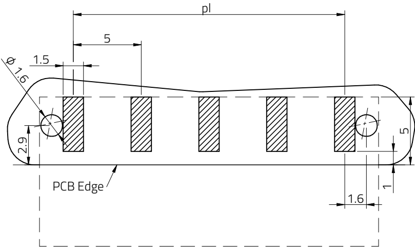
Recommended layout only for coding OA
