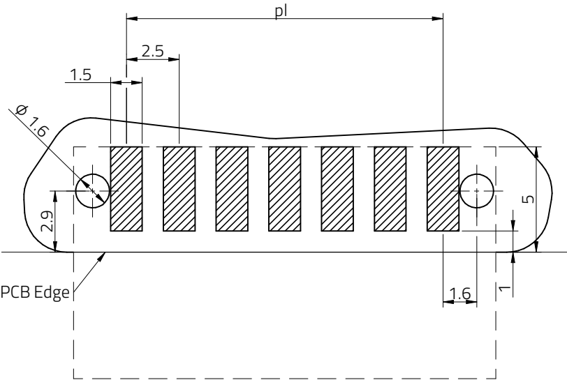
Recommended layout only for coding 0A
