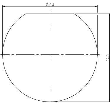
Recommended Mounting Hole Max Panel Thickness = 5 mm
