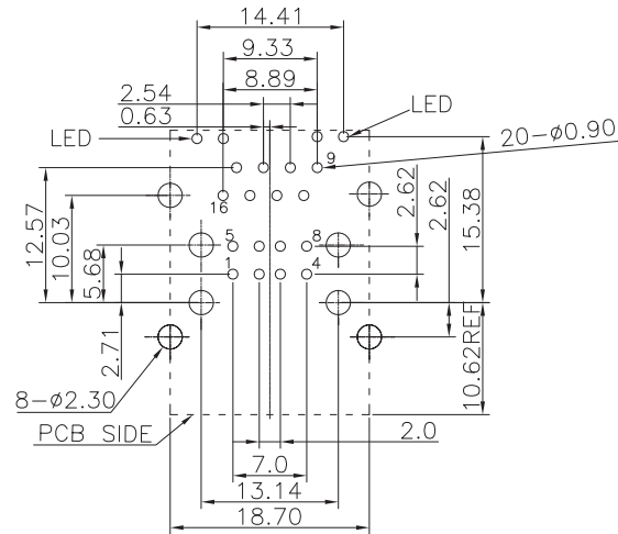
PCB LAYOUT COMPONENT VIEW TOLERANCE: \pm 0.05\text{mm}
