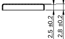
sectional drawing A-A
