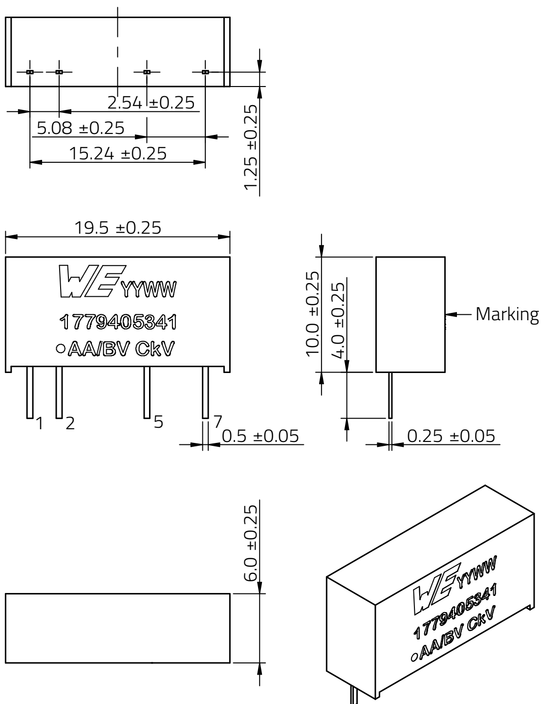
Figure 19: Component dimensions.
