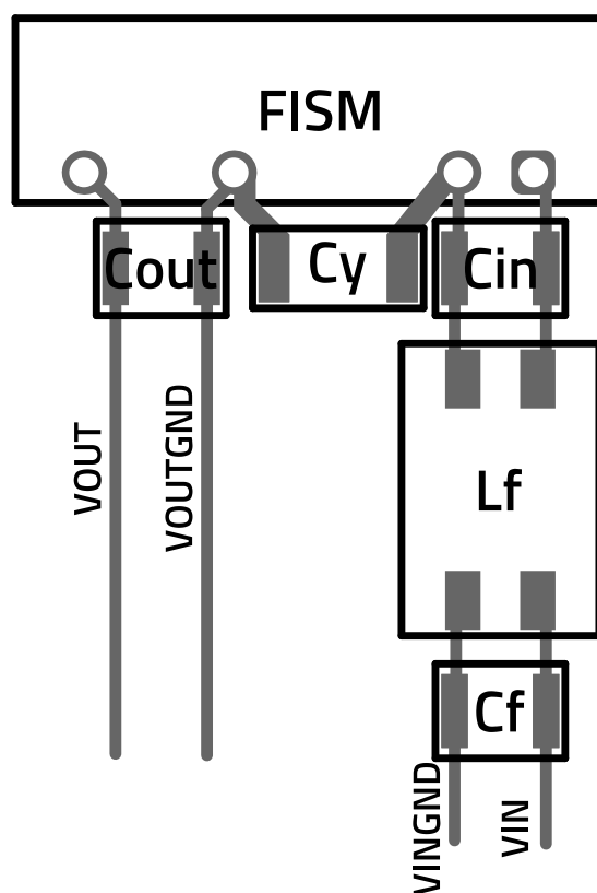
Figure 12: Layout recommendation.
