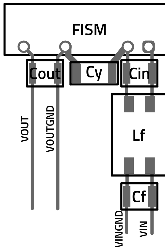
Figure 12: Layout recommendation.
