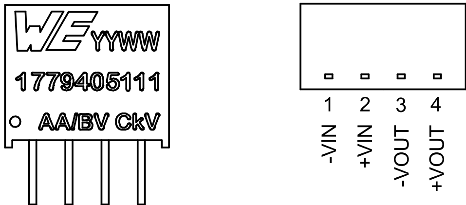
Figure 1: Pinout.
