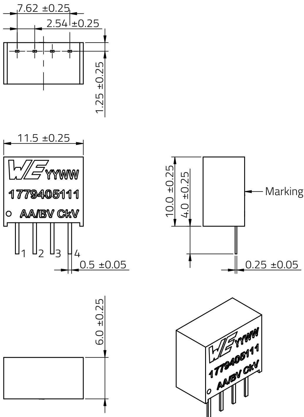
Figure 19: Component dimensions.
