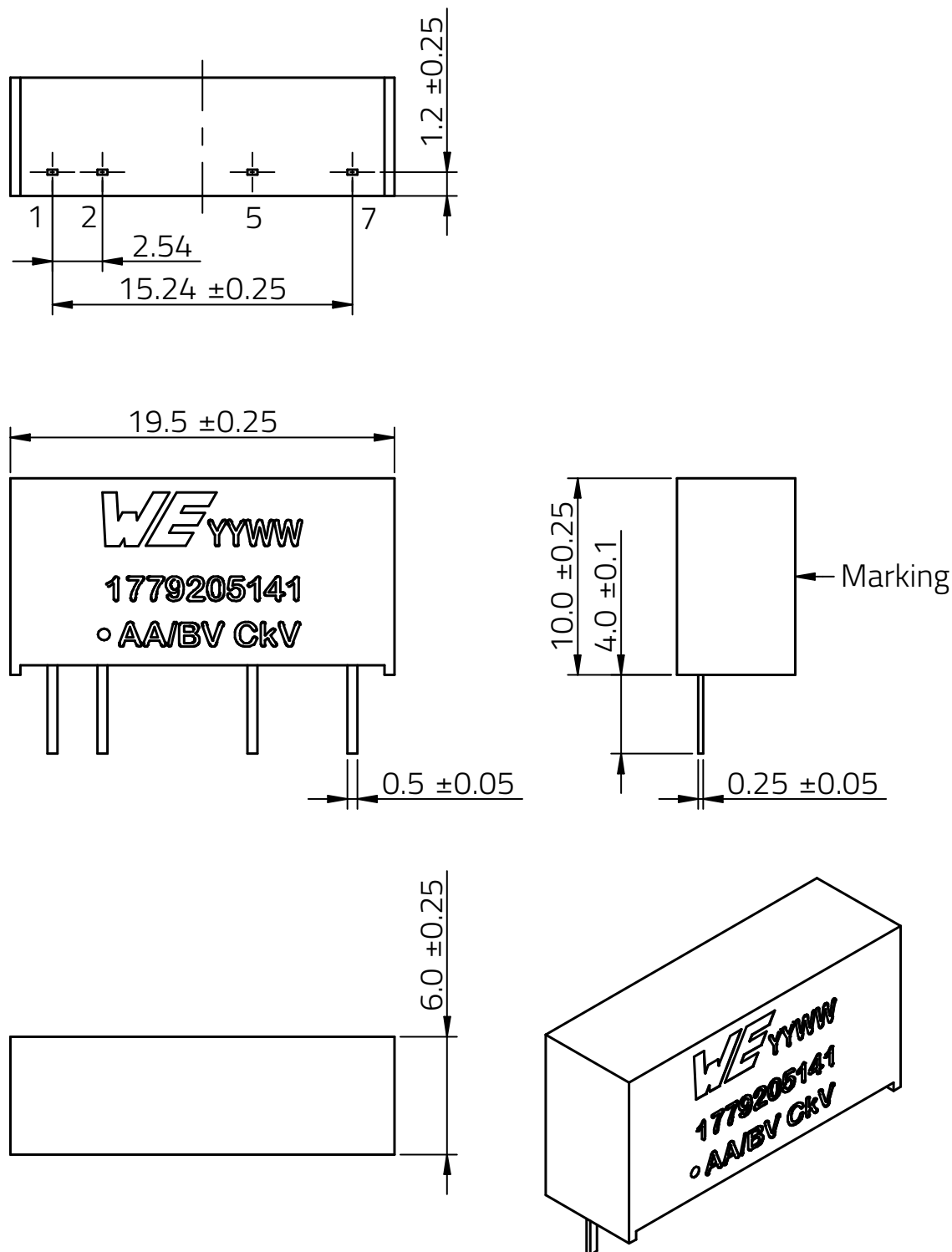
Figure 19: Component dimensions.
