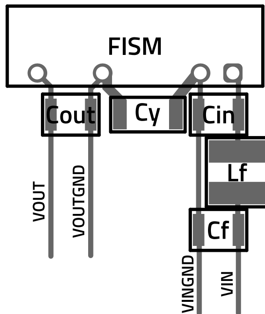
Figure 12: Layout recommendation.
