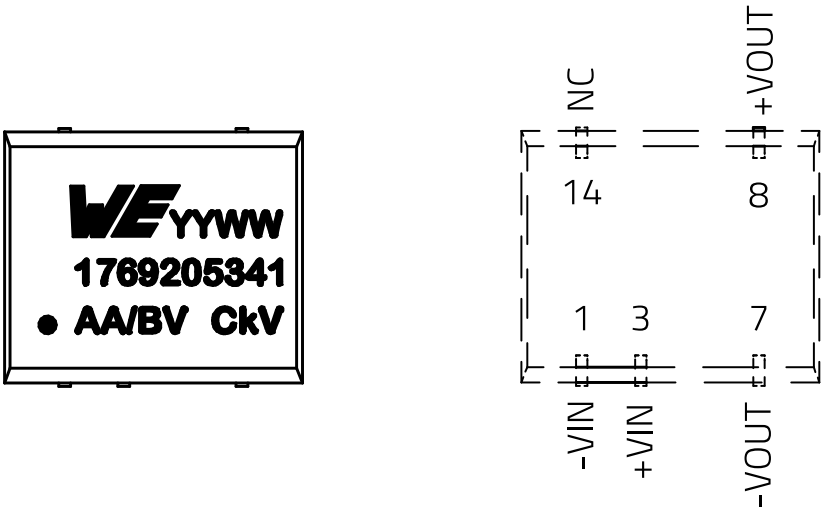
Figure 1: Pinout.
