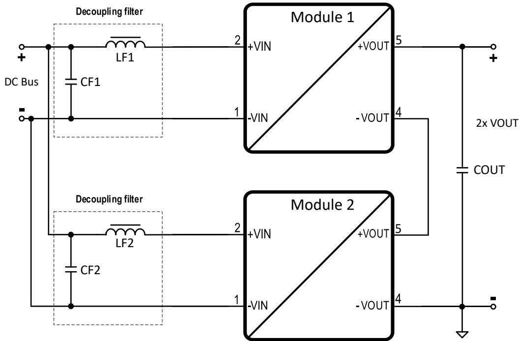
Figure 14: Primary side serial connection.
