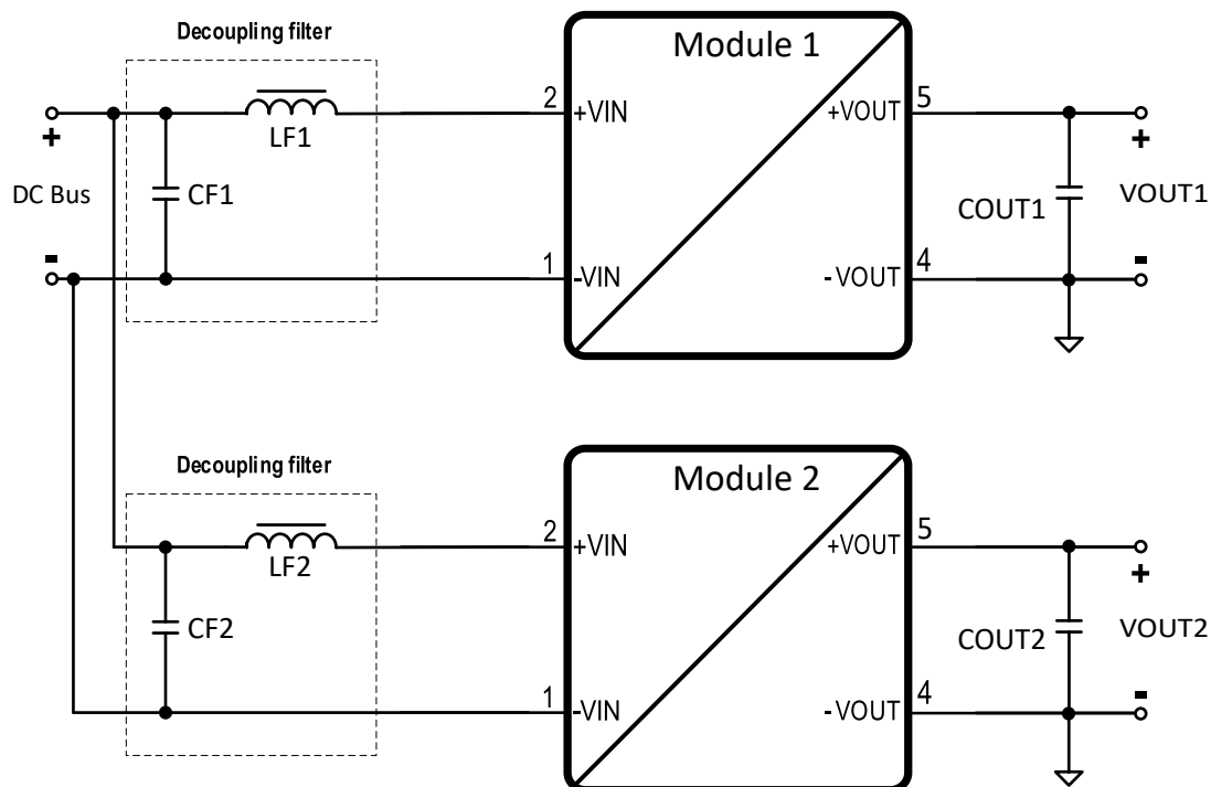
Figure 13: Decoupling for primary side parallel connection.
