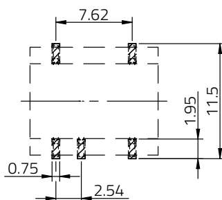
Figure 19: Recommended landpattern dimensions.
