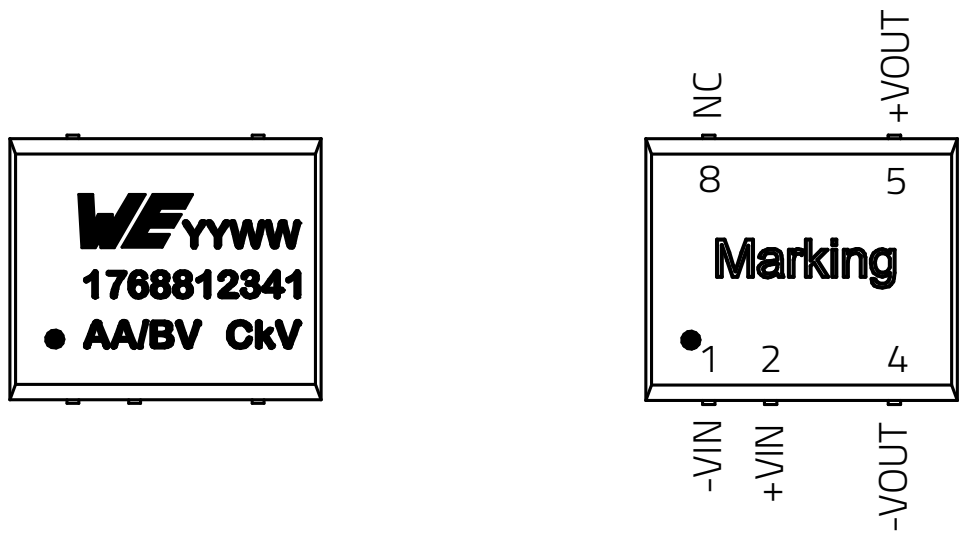
Figure 1: Pinout.
