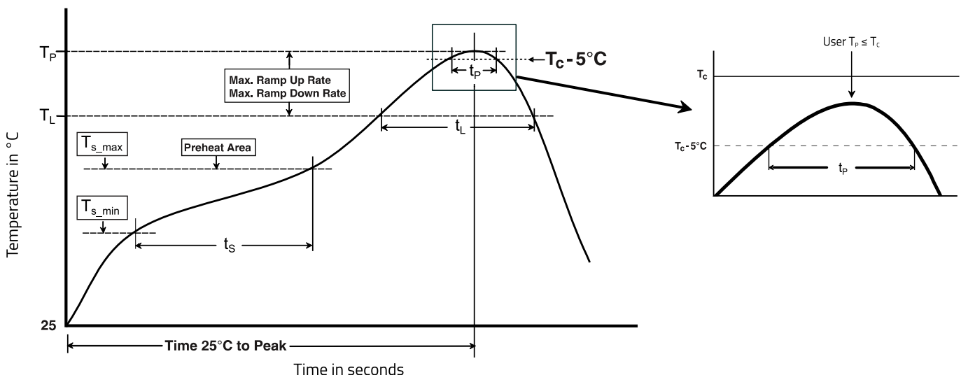
Figure 17: Solder profile.
