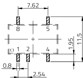
Figure 19: Recommended landpattern dimensions.
