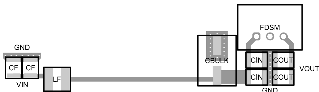
Figure 13: Layout recommendation.
