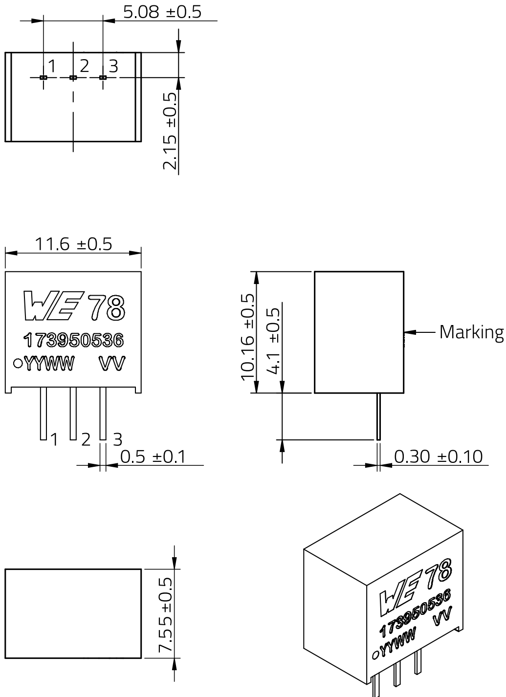
Figure 18: Physical dimensions.
