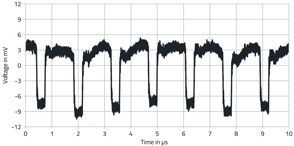
Figure 9: Output voltage ripple, V_{IN} = 24V , I_{OUT} = 0.5A .
