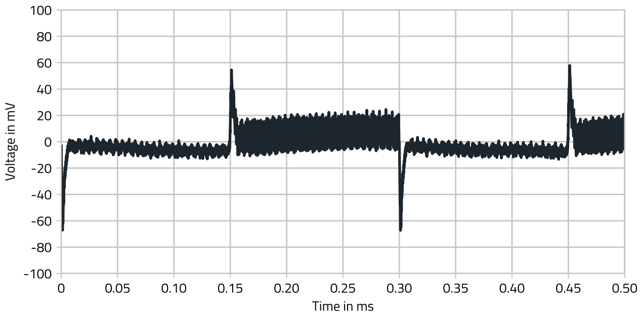
Figure 12: 171030560 V_{IN} = 5V , V_{OUT} = 3.3V , load jumps 0% - 100%.
