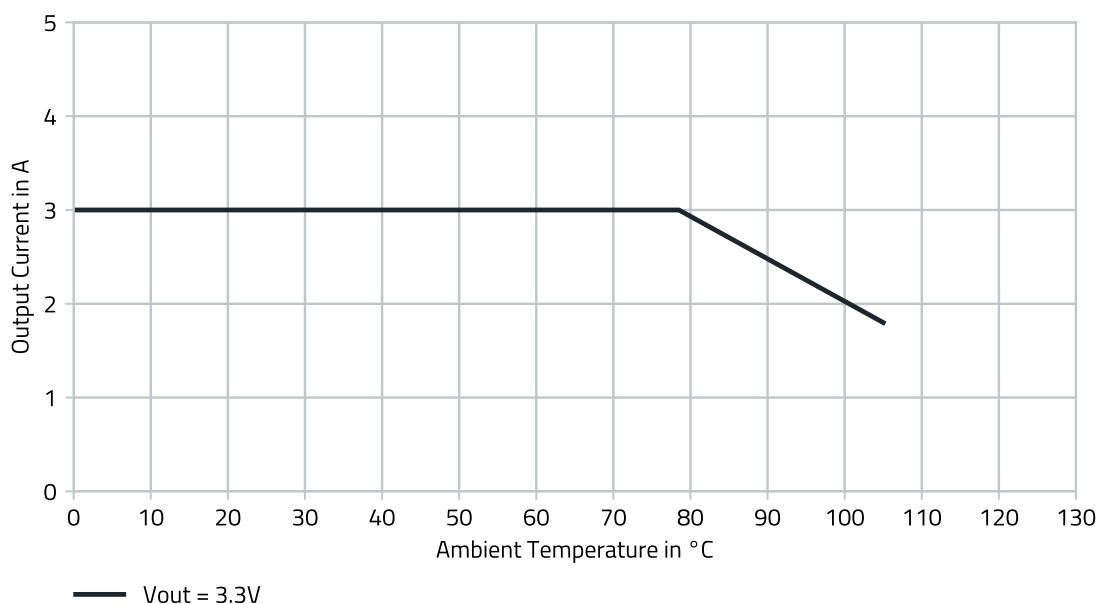
Figure 5: 171030560 output current thermal derating V IN = 5V.
