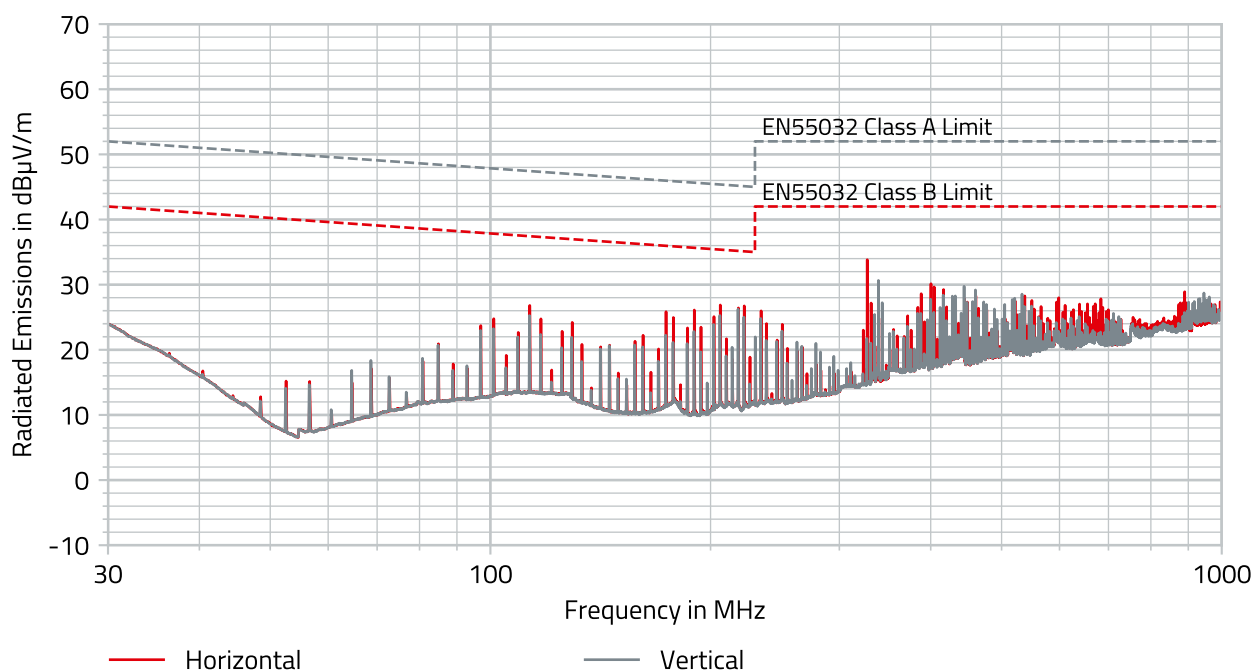
Figure 2: Radiated emissions 171030560 V_{IN} = 5\text{V} , V_{OUT} = 3.3 , I_{LOAD} = 3\text{A} with input filter.
