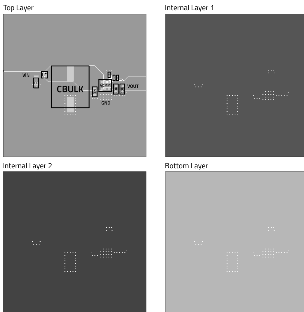
Figure 19: 171030560 layout recommendation.
