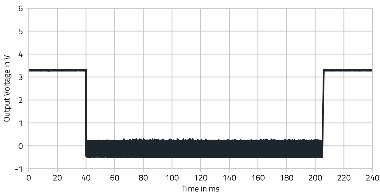
Figure 16: 171030560 short circuit protection V_{IN} = 5V , V_{OUT} = 3.3V .
