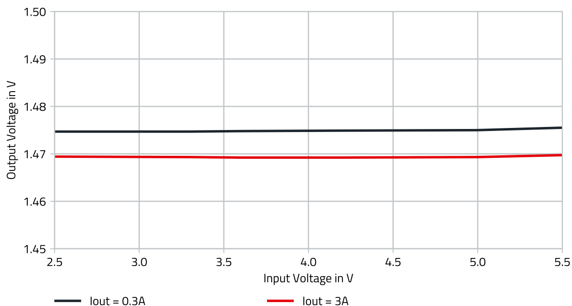
Figure 8: 171030560 Load Regulation V_{OUT} = 3.3V .
