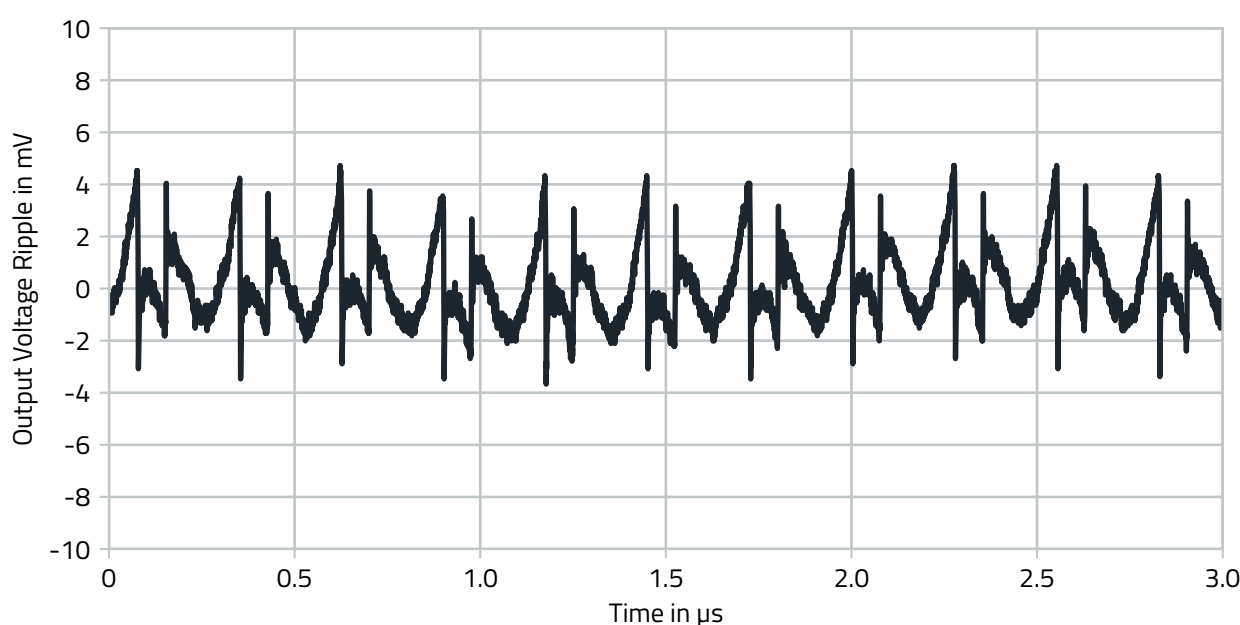
Figure 14: 171030560 output voltage ripple V_{IN} = 5V , V_{OUT} = 3.3V , I_{OUT} = 3A .
