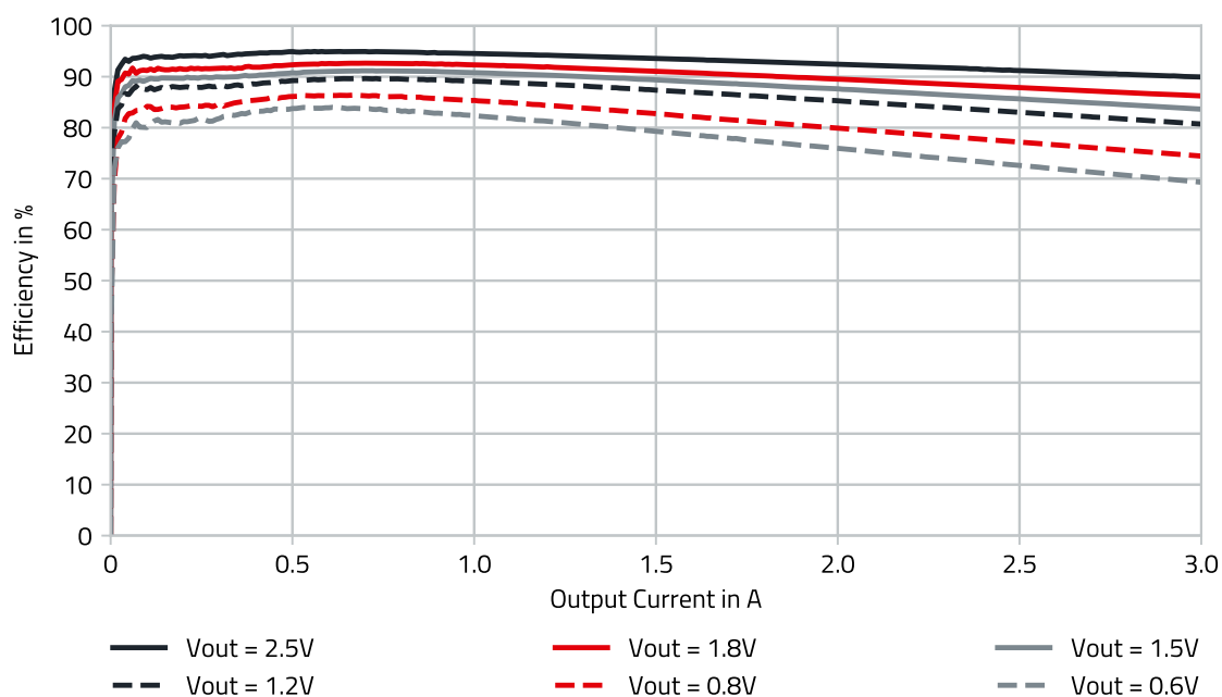
Figure 4: 171030560 efficiency V_{IN} = 3.3V .
