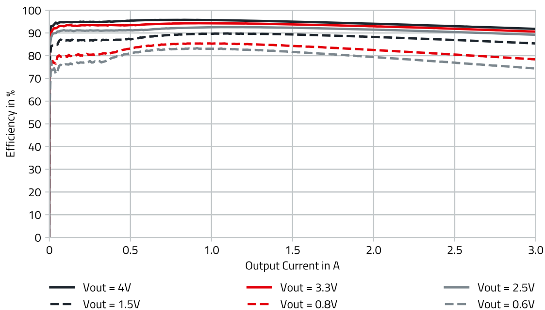
Figure 3: 171030560 efficiency V_{IN} = 5V .
