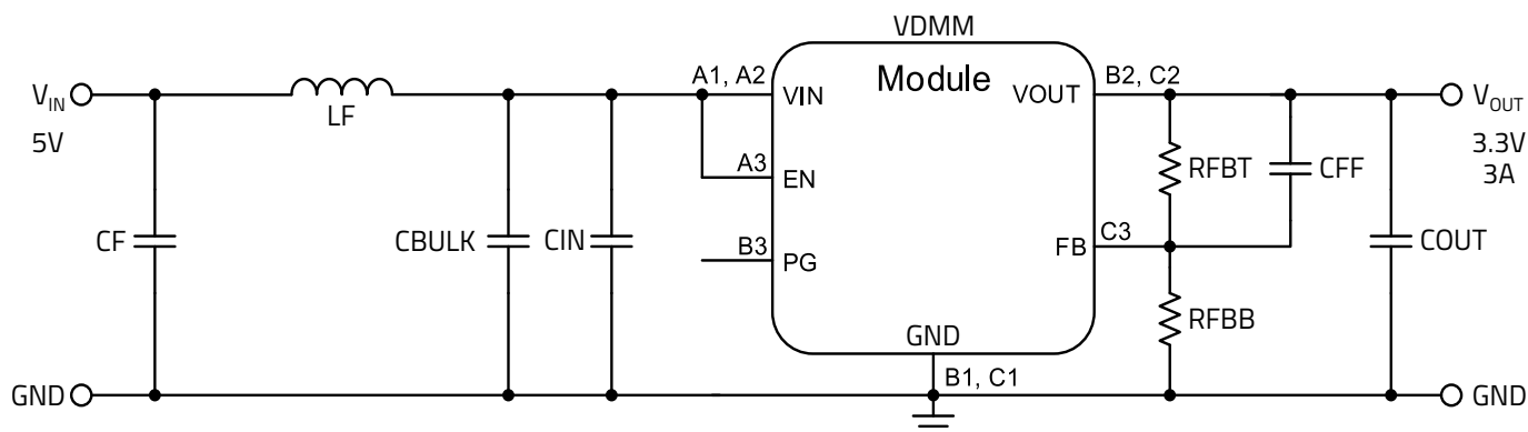
Figure 20: 171030560 design example schematic.
