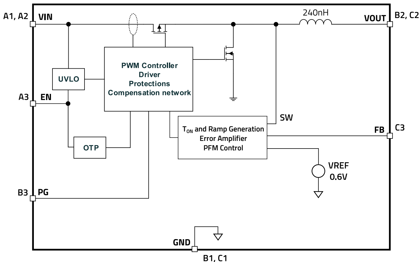
Figure 9: 171030560 block diagram.
