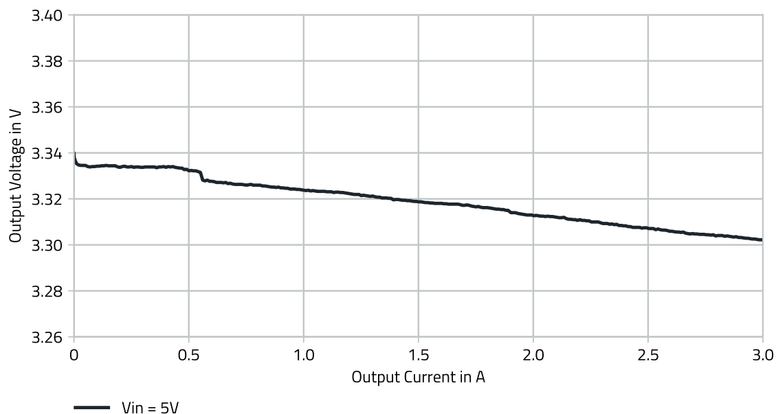
Figure 6: 171030560 Load Regulation V OUT = 3.3V.
