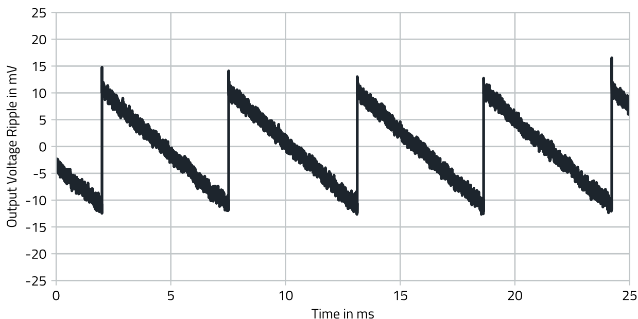
Figure 13: 171030560 output voltage ripple V_{IN} = 5V , V_{OUT} = 3.3V , I_{OUT} = 0A .
