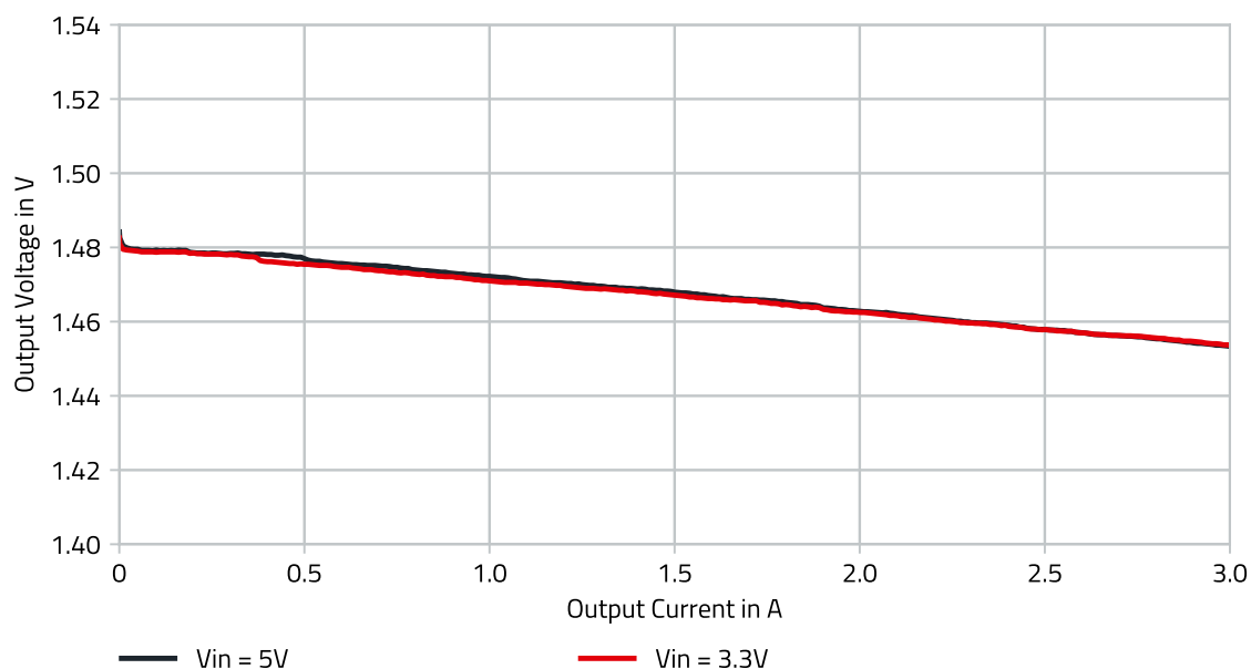
Figure 7: 171030560 Load Regulation V_{OUT} = 1.5V .
